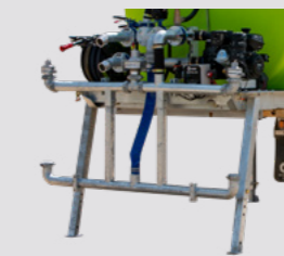
Self-Loading Legs
